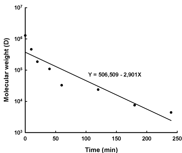
Fig. 2. Correlationship between the molecular weight of partially hydrolyzed alginate at 100°C and reaction time with acetic acid.
