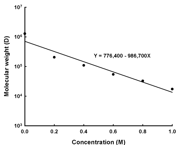
Fig. 1. Correlationship between the molecular weight of partially hydrolyzed alginate at 100°C for 40 min and concentration of acetic acid.
