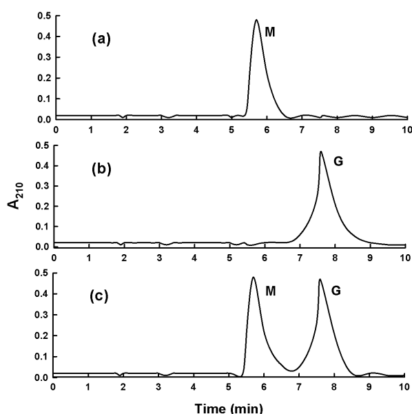
Fig. 4. High performance liquid chromatograms of (a) D-mannuronate lactone (M), (b) L-gulonate lactone (G) and (c) mixture of D-mannuronate lactone and L-gulonate lactone (1 : 1) eluted with 20 mM \text{KH}_2\text{PO}_4 (pH 4.6) containing 5% methanol at a flow rate of 1.0 ml/min.
